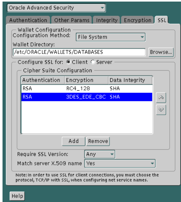
Figure 7-6 Oracle Advanced Security SSL Window (Client)
