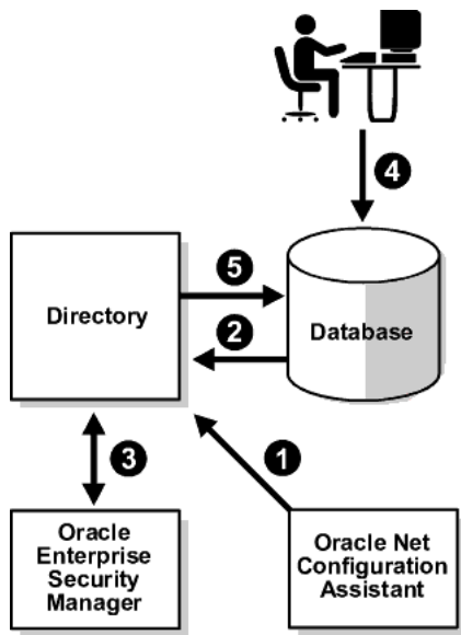
Figure 15–4 How Enterprise User Security Works
