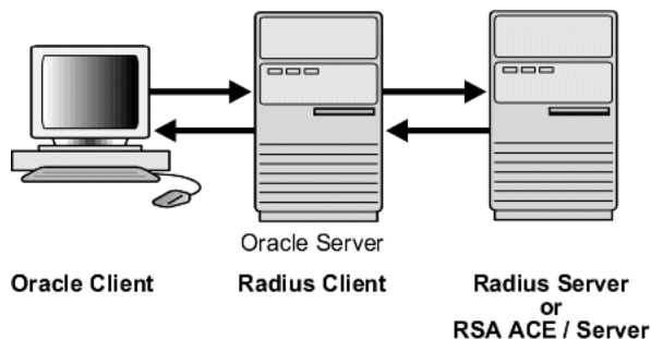
Figure 4-1 RADIUS in an Oracle Environment
