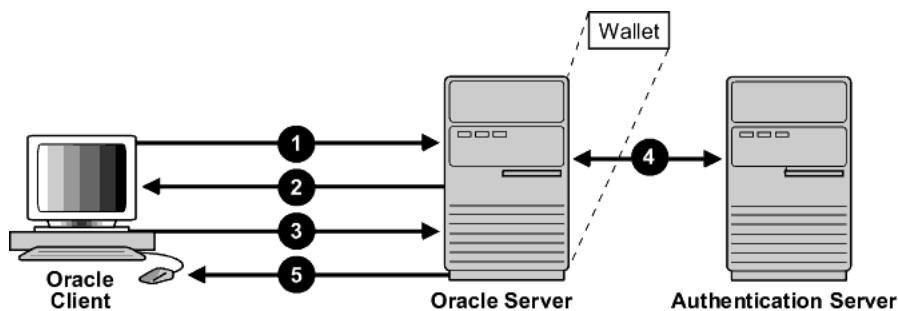
Figure 7-3 SSL in Relation to Other Authentication Methods
