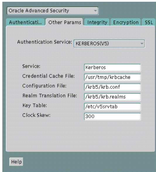
Figure 6–2 Oracle Advanced Security Other Params Window (Kerberos)
