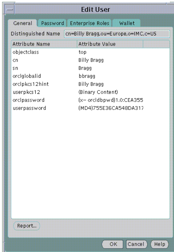
Figure 19–8 Oracle Enterprise Security Manager: Edit User Window
