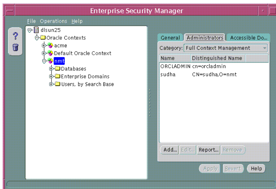
Figure 19–11 Oracle Enterprise Security Manager Administrator's Tab
