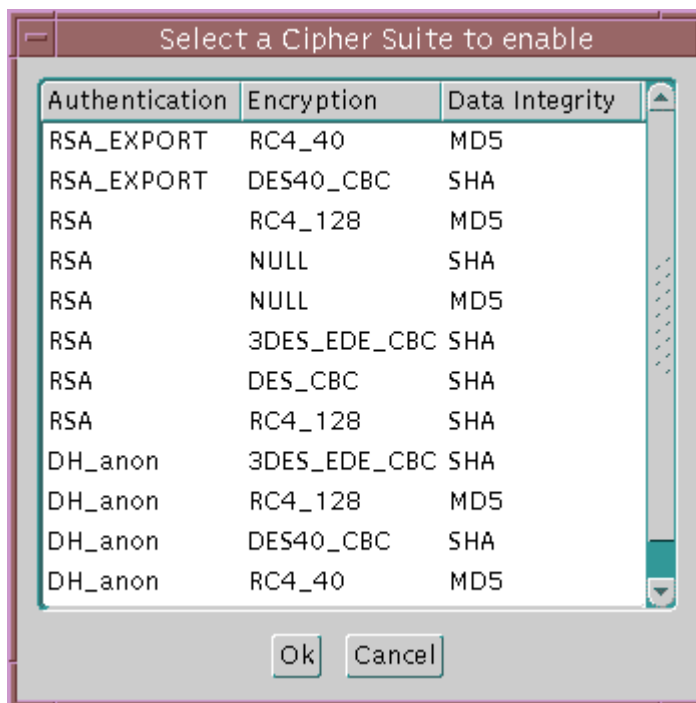
Figure 7-5 SSL Cipher Suites Window
