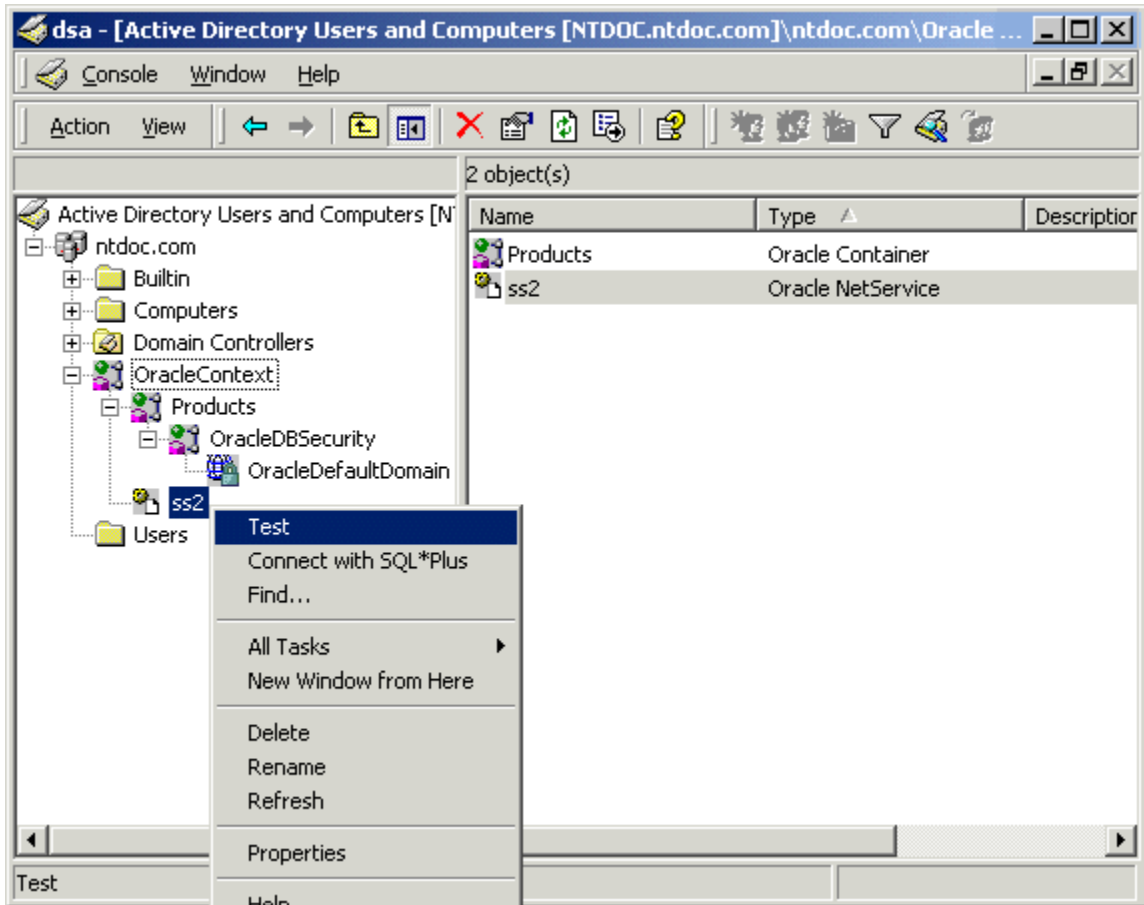
Figure E-1 Directory Object Type Descriptions in Active Directory
