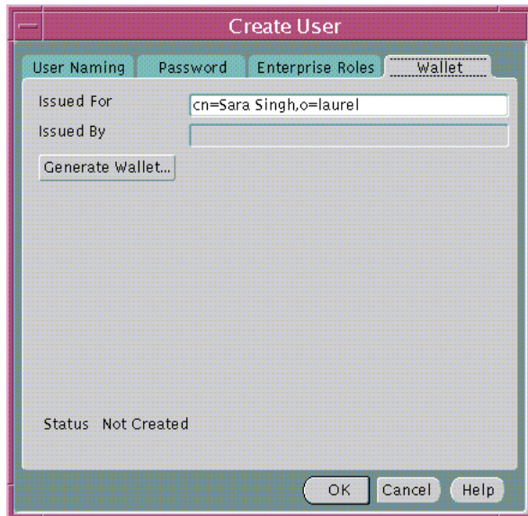
Figure 19–6 Oracle Enterprise Security Manager: Create User Window (Wallet Tab)
