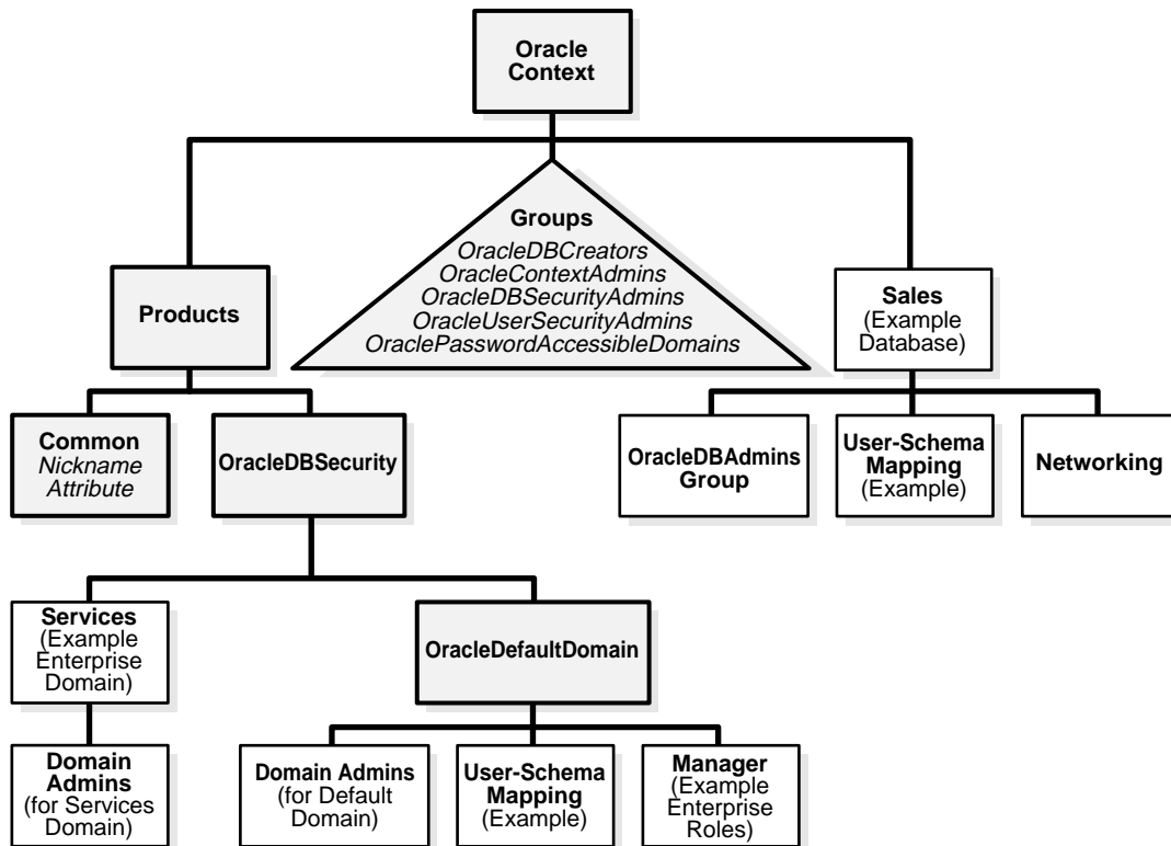
Figure 15–1 Related Entries in an Oracle Context
