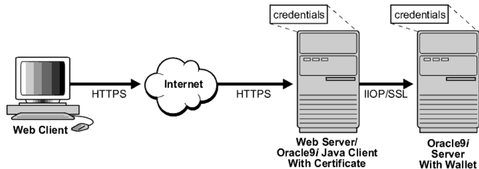
Figure 7-1 Connecting to an Oracle Server over the Internet
