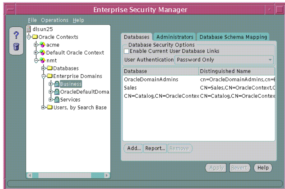
Figure 19–16 Oracle Enterprise Security Manager: Databases Tab (Database Membership)
