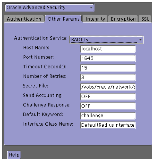
Figure 4-5 Oracle Advanced Security Other Params Window
