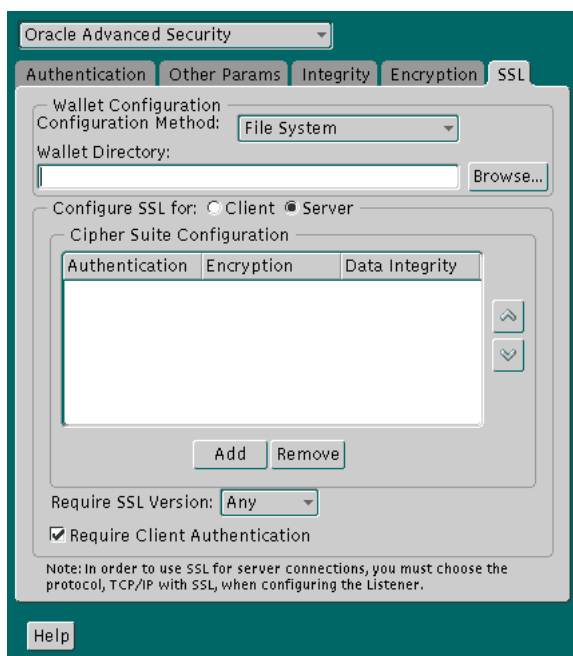
Figure 7–8 Oracle Advanced Security SSL Window (Server)
