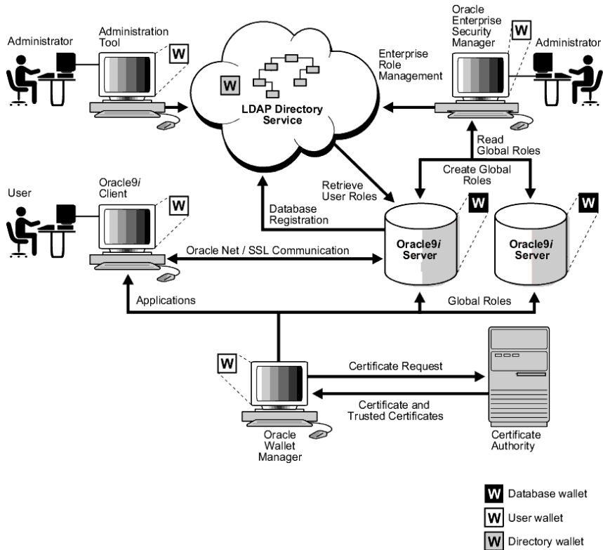
Figure 15-2 Enterprise User Security Elements (SSL-Authentication)
