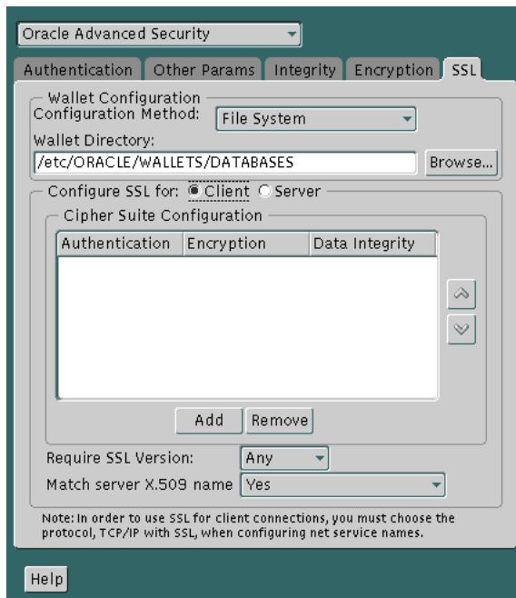
Figure 7–4 Oracle Advanced Security SSL Window (Client)
