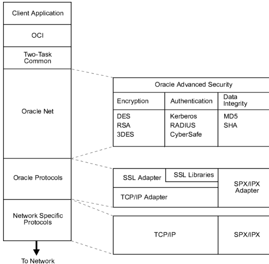
Figure 7-2 SSL in Relation to Oracle Advanced Security
