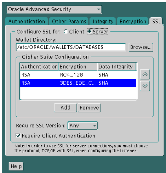
Figure 7-7 Oracle Advanced Security SSL Window (Server)
