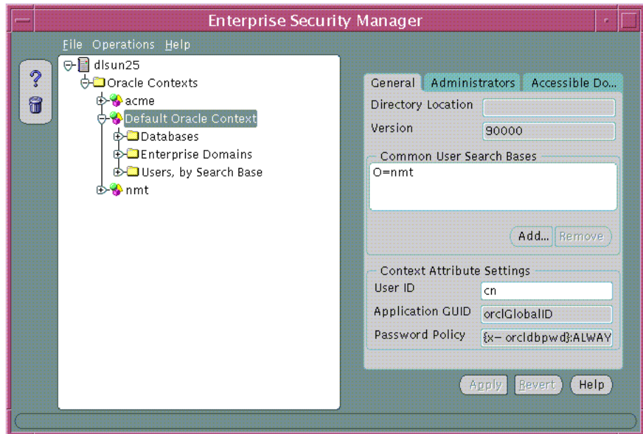
Figure 19–9 Oracle Enterprise Security Manager: General Tab
