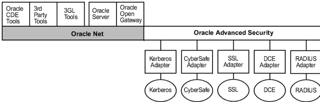
Figure 1–3 Oracle Net with Authentication Adapters
