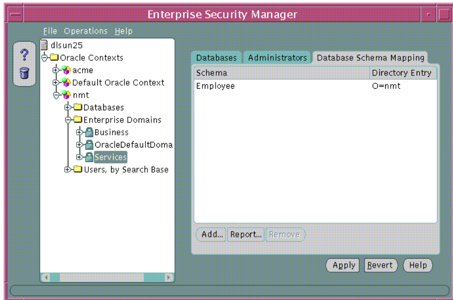
Figure 19–18 Oracle Enterprise Security Manager: Database Schema Mappings Tab
