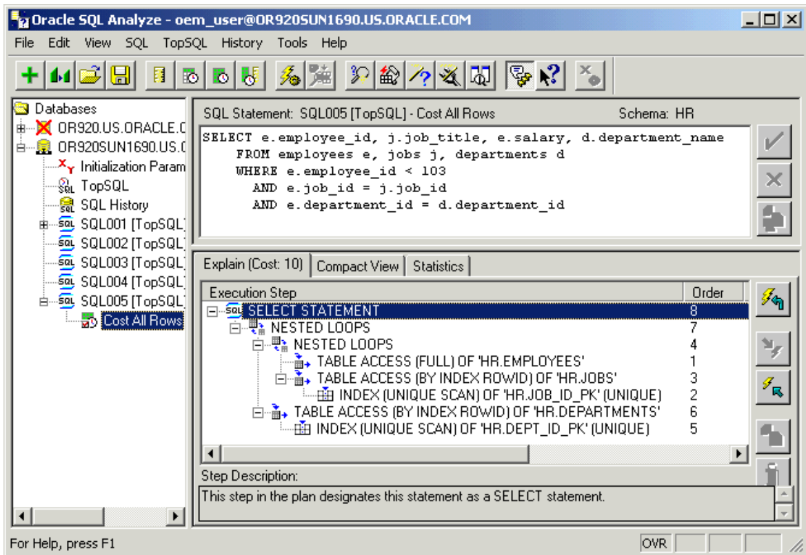
Figure 6–1 Oracle SQL Analyze
