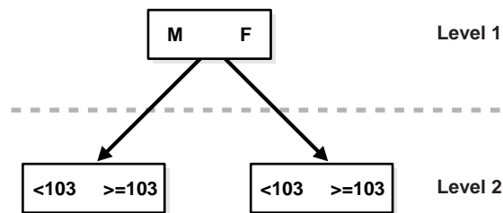
Figure 1–4 Index Skip Scan Illustration
