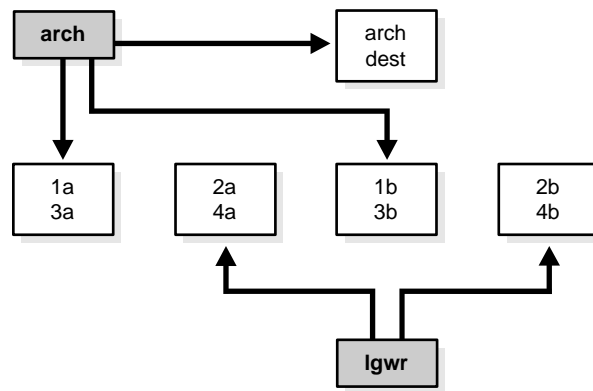
Figure 15–1 Distributing Redo Members Across Disks
