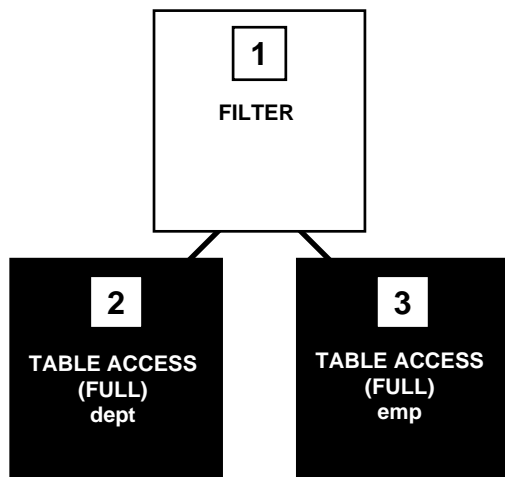
Figure 8–1 Execution Plan with Two Full Table Scans
