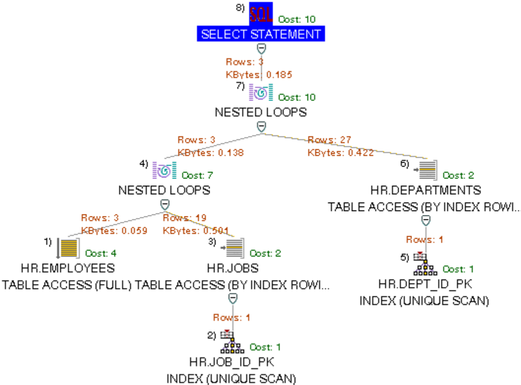
Figure 1-3 Graphical View of SQL Explain Plan in SQL Scratchpad
