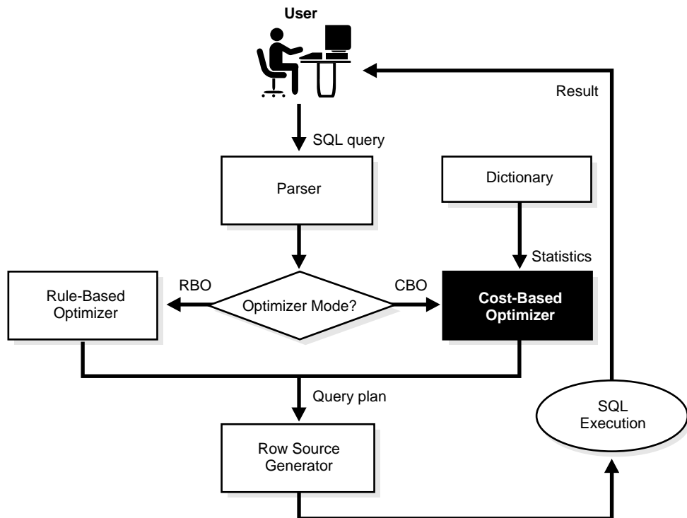
Figure 1-1 SQL Processing Overview
