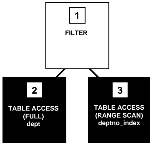
Figure 8–2 Execution Plan with a Full Table Scan and an Index Scan
