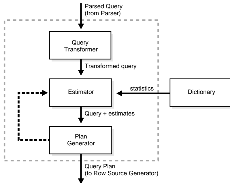
Figure 1-2 Cost-Based Optimizer Components
