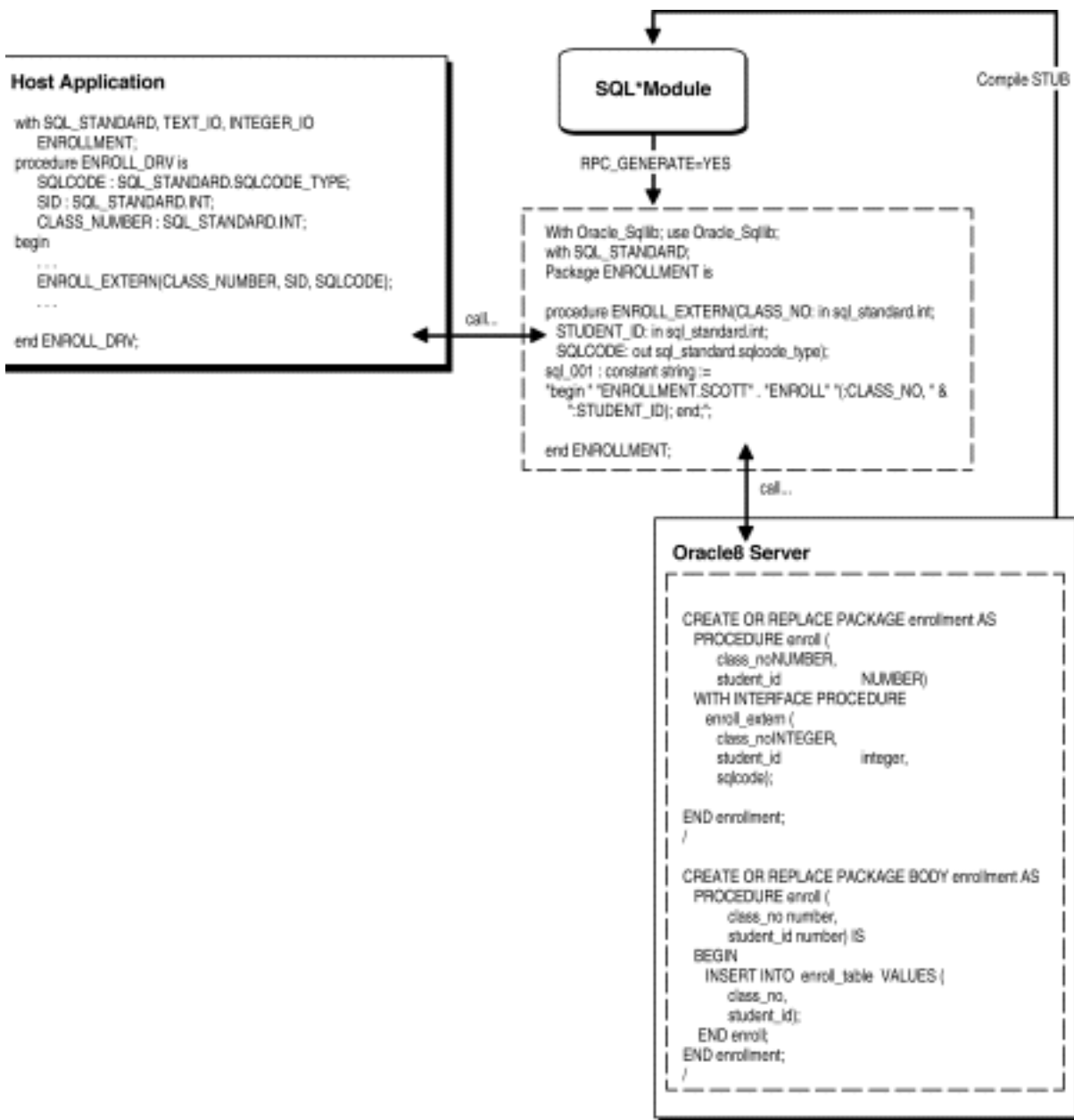
Figure 3-1 Accessing a Stored Procedure
