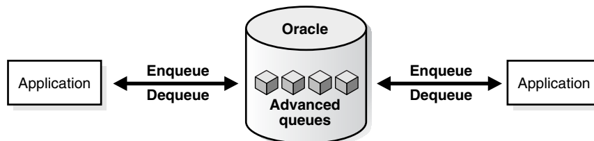
Figure 1–6 Point-to-Point Messaging
