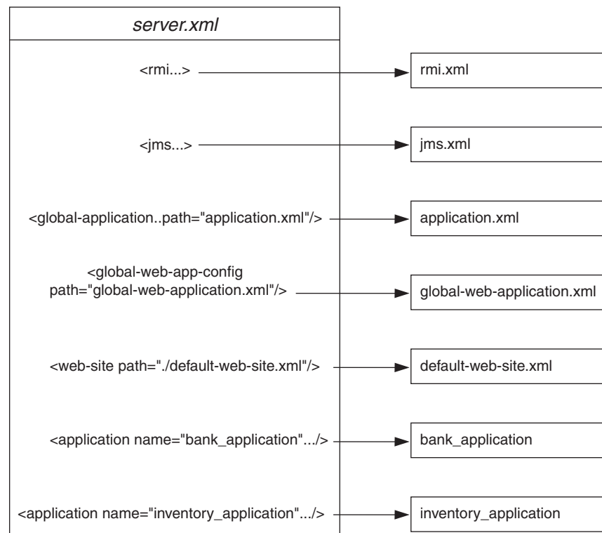
Figure 3-17 Server.xml File and Related XML Files
