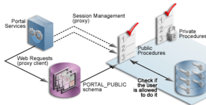
Figure 6–15 N-Tier Authentication By User Proxy
