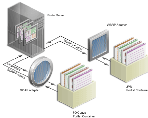
Figure 6–21 OracleAS Portal's WSRP Architecture
