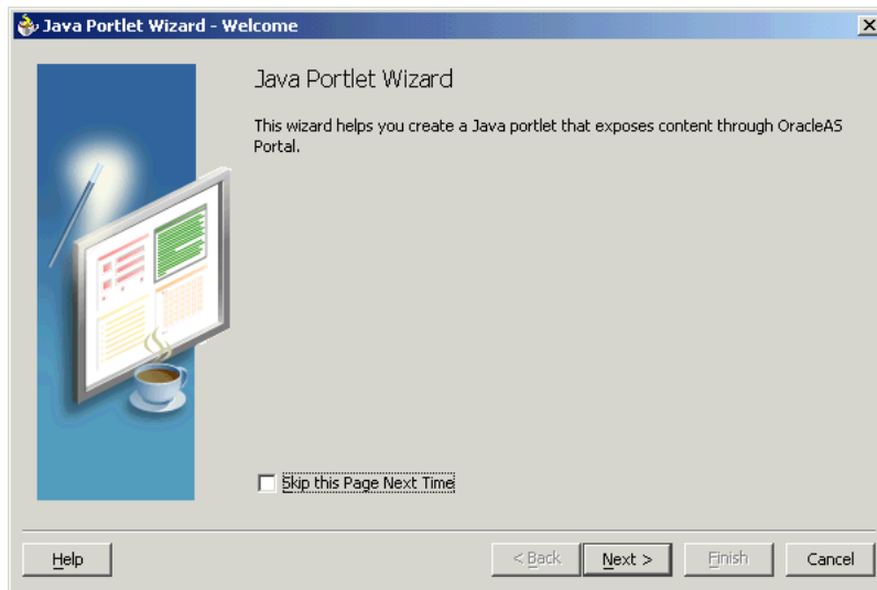
Figure 6–33 Welcome Page
