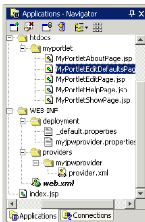
Figure 6–41 Application Navigator
