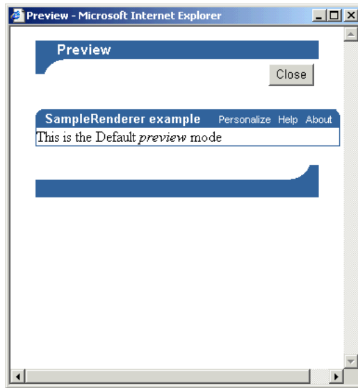
Figure 7-3 Preview Window
