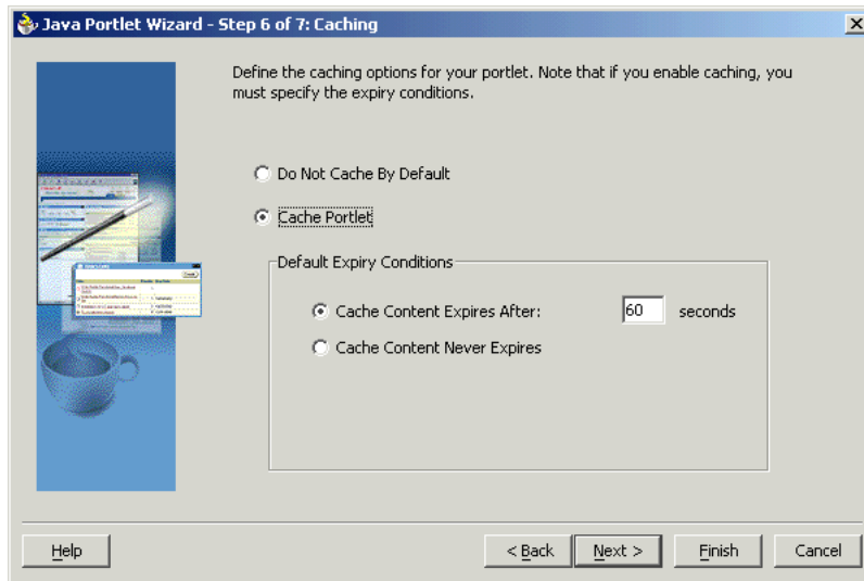
Figure 6–25 Caching Page
