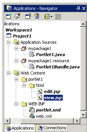
Figure 6–27 Application Navigator
