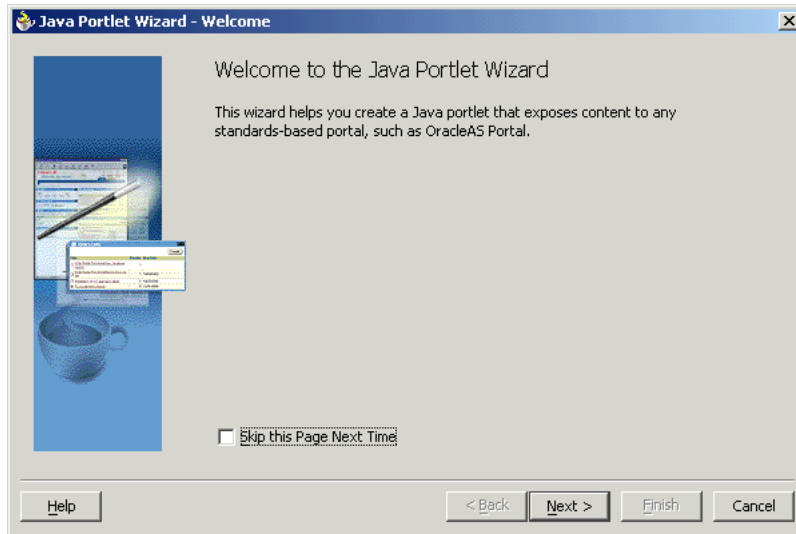
Figure 6–17 Welcome Page
