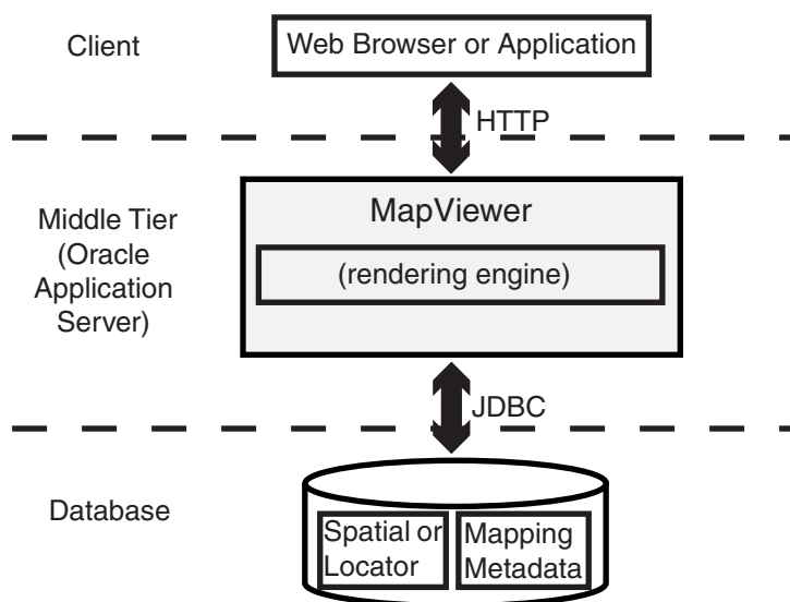
Figure 1–2 OracleAS MapViewer Architecture
