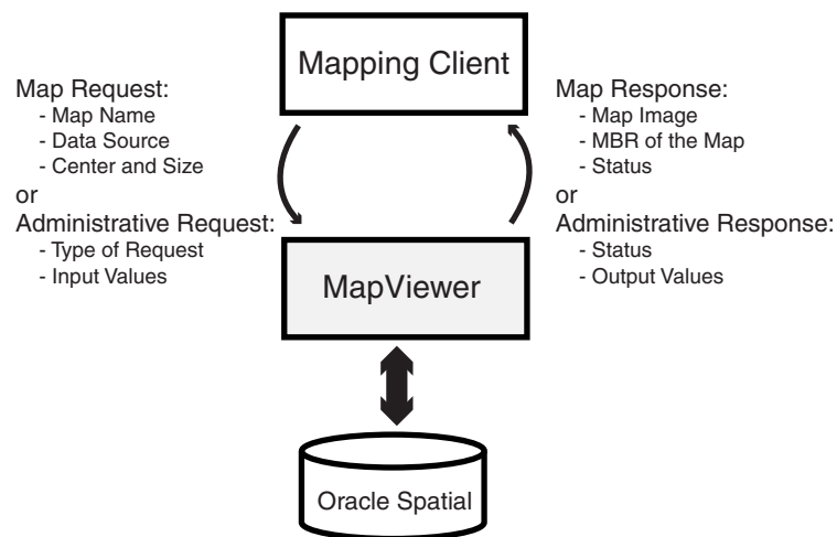
Figure 1–1 Basic Flow of Action with OracleAS MapViewer
